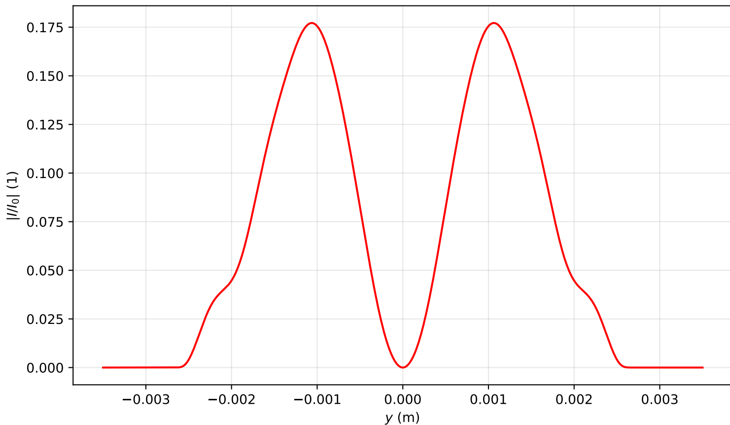
Intensity profile I(x=0, y, z=3.901)/I_0 , P_{in}=0.5P_{cr} , artificial time
